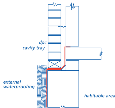
Example of linking waterproofing with DPC/cavity tray
